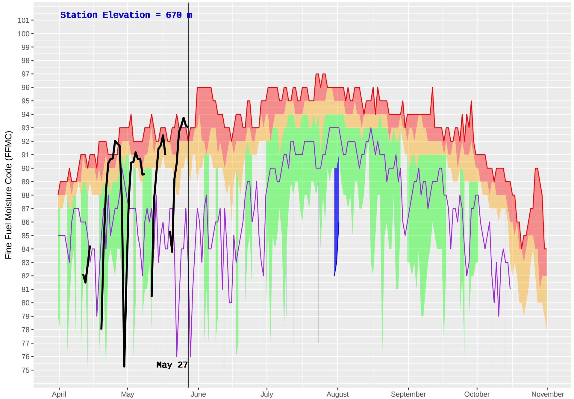
FINTRY (298) : Historical (1989–2016) and Current (2018) Noon Fine Fuel Moisture Code (FFMC)
