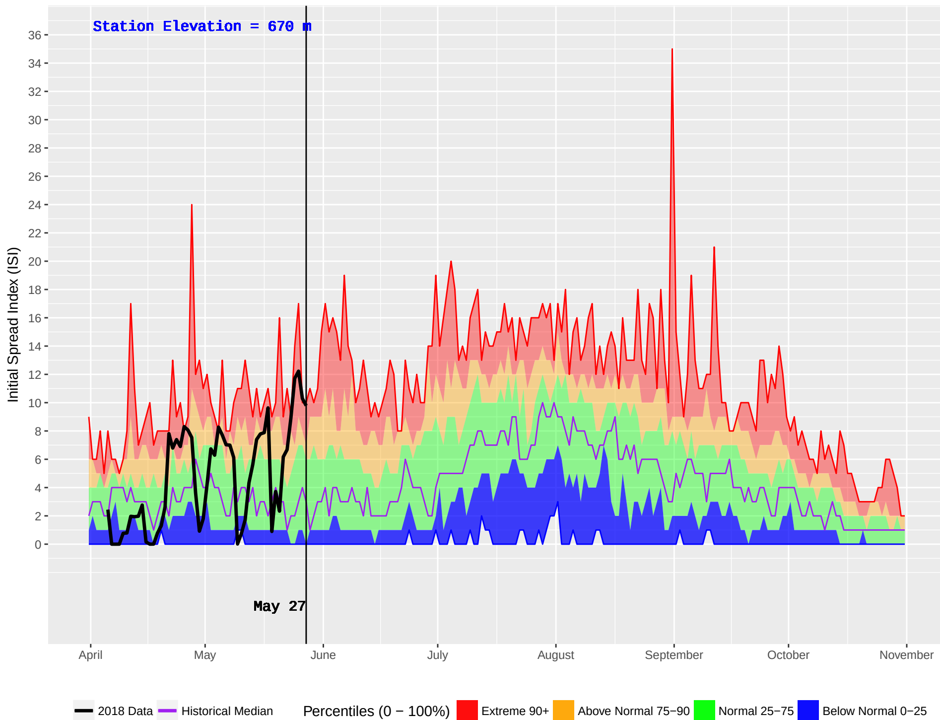
FINTRY (298) : Historical (1989–2016) and Current (2018) Noon Initial Spread Index (ISI)
