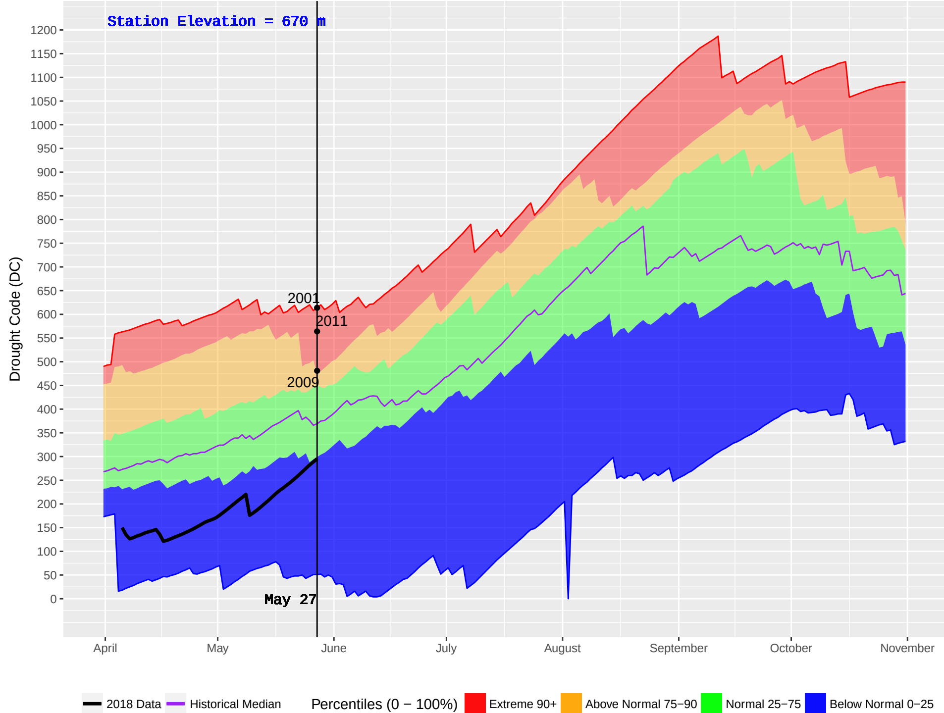
FINTRY (298) : Historical (1989–2016) and Current (2018) Noon Drought Code (DC)
