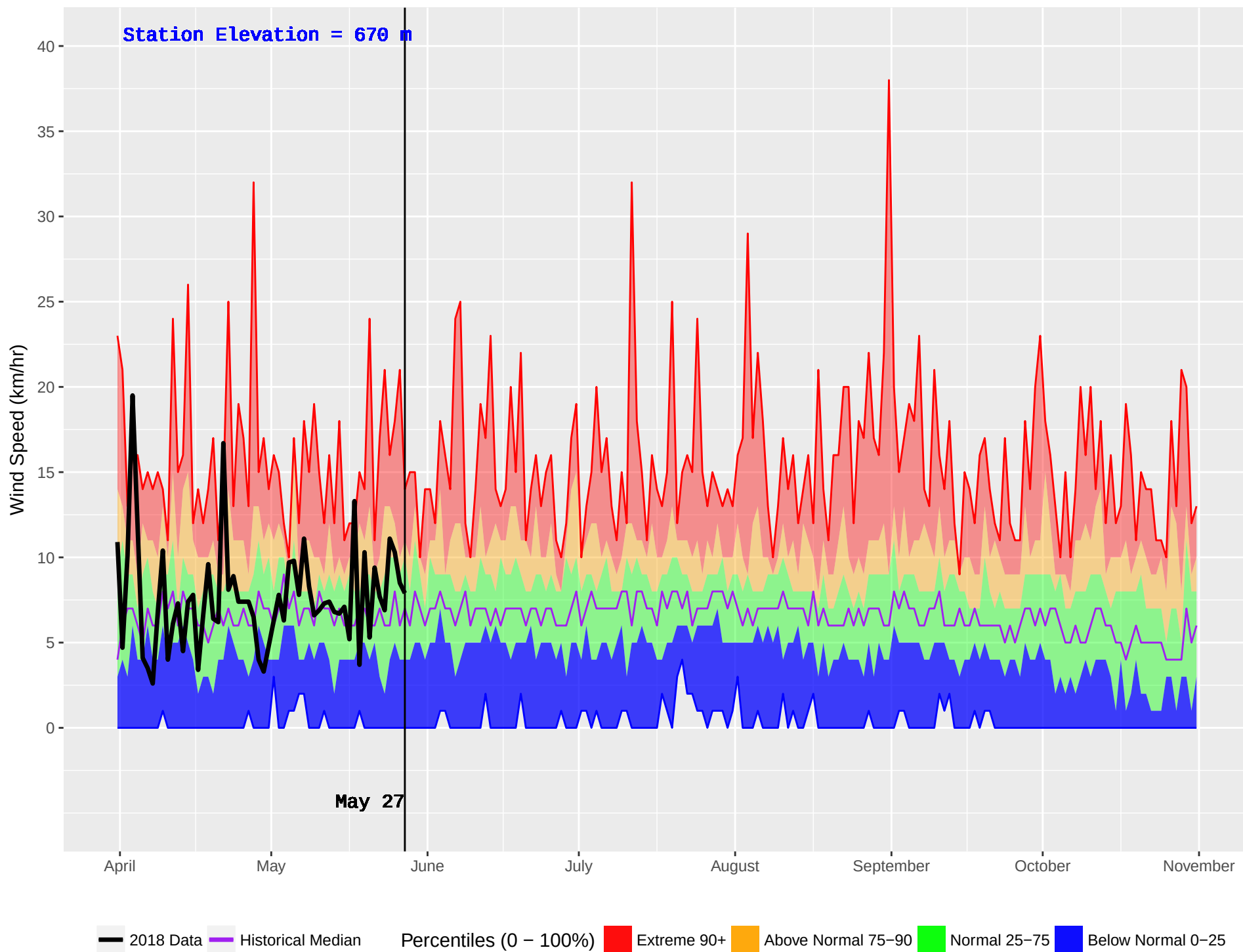
FINTRY (298) : Historical (1989–2016) and Current (2018) Noon Wind Speed
