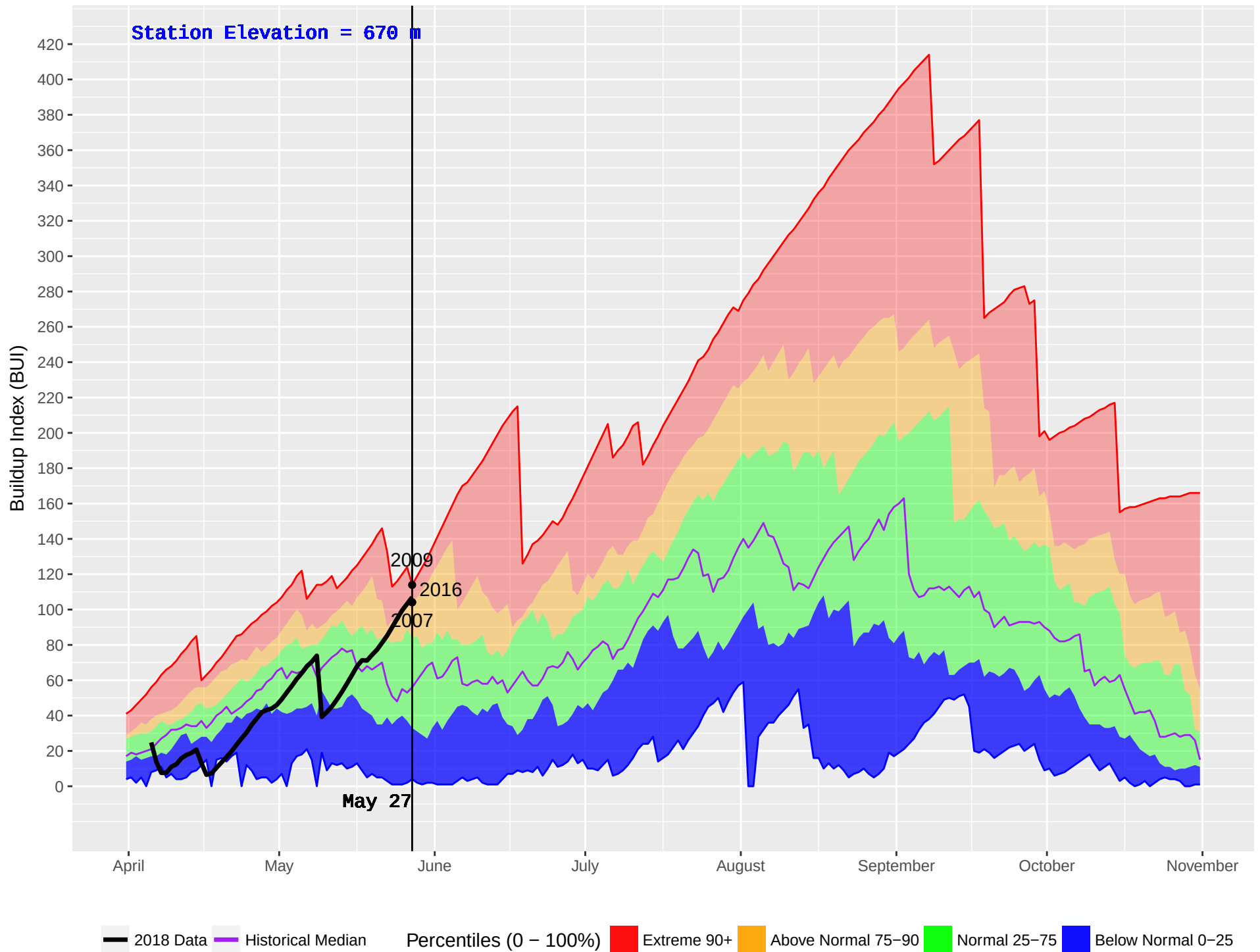
FINTRY (298) : Historical (1989–2016) and Current (2018) Noon Buildup Index (BUI)
