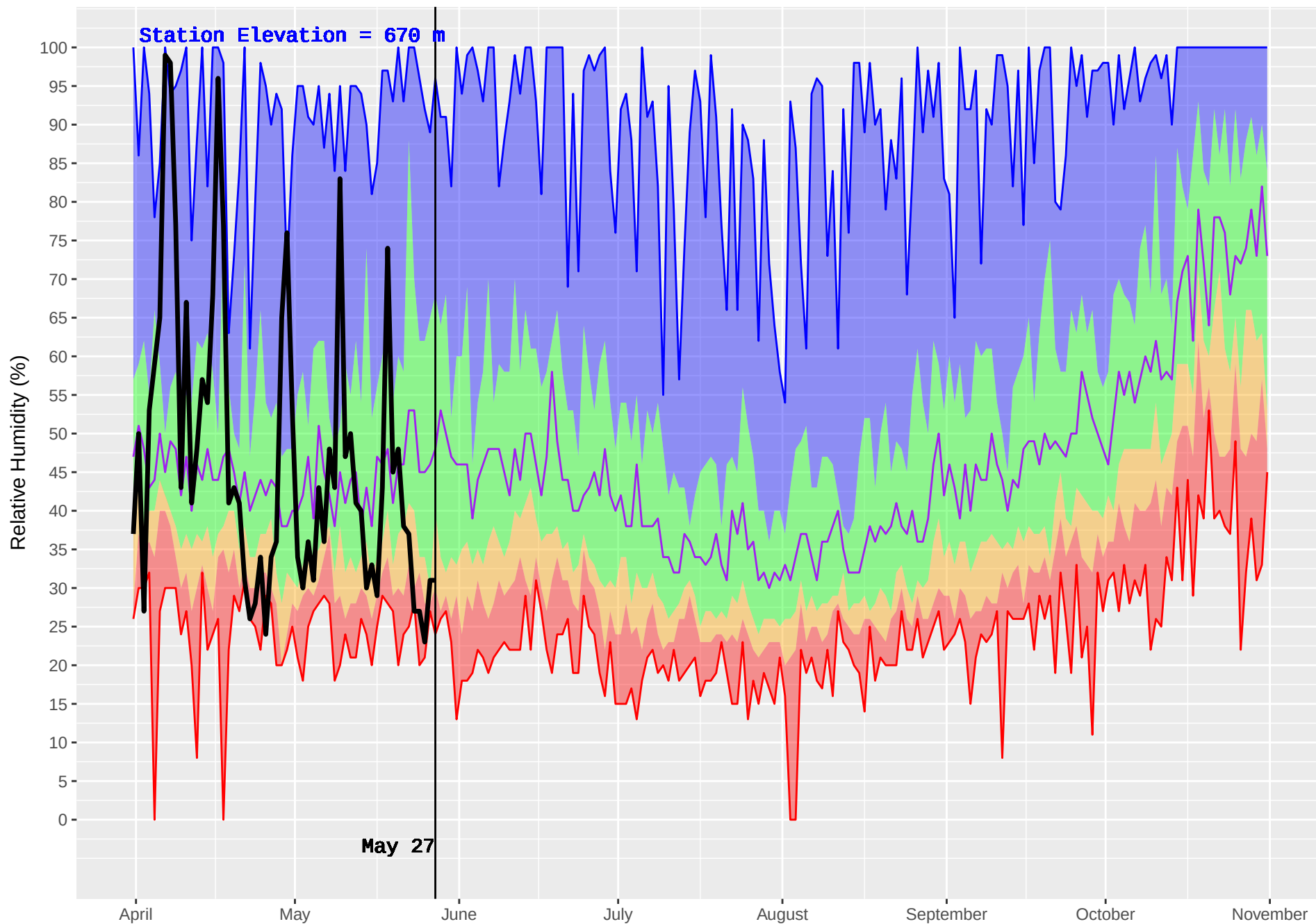
FINTRY (298) : Historical (1989–2016) and Current (2018) Noon Relative Humidity
