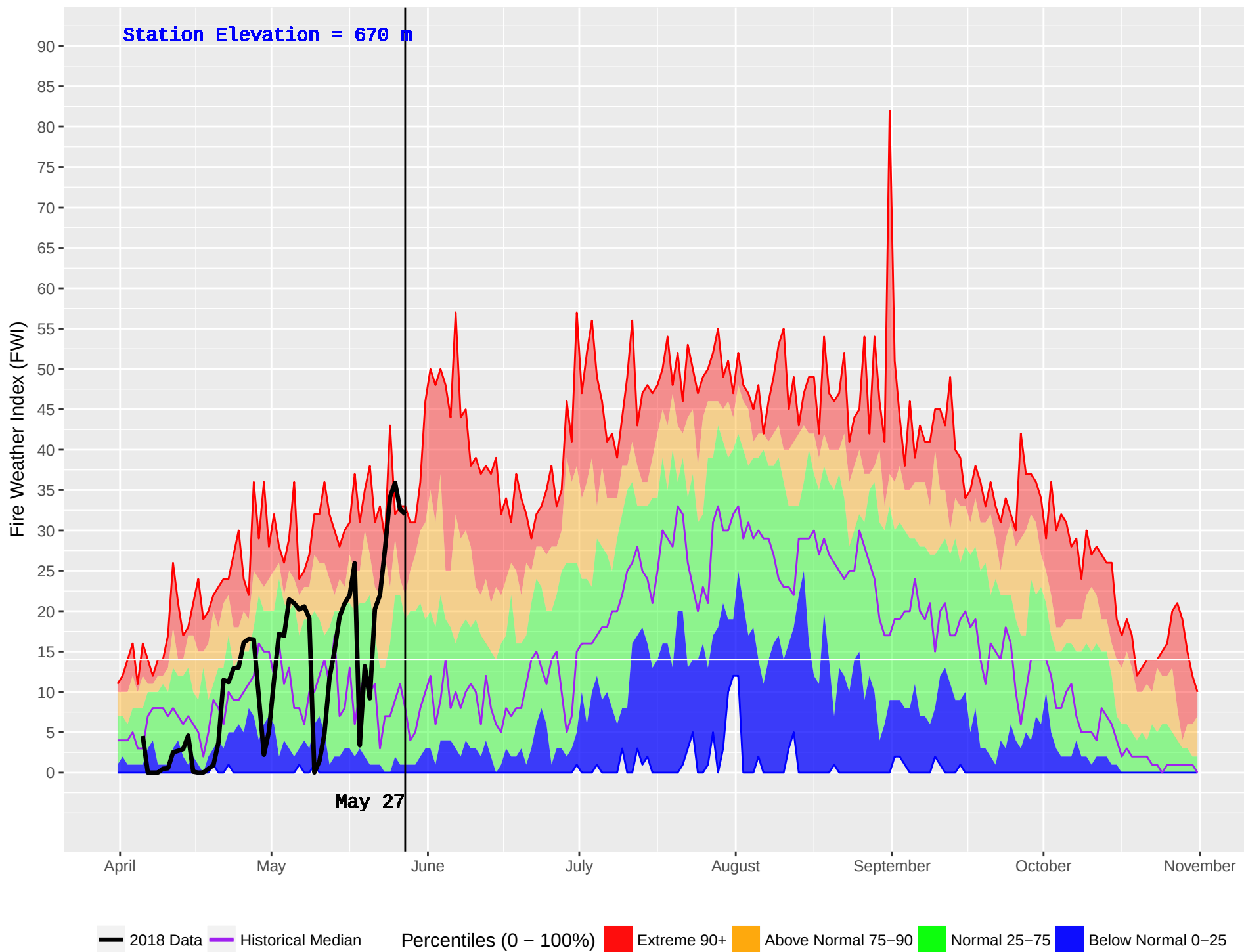
FINTRY (298) : Historical (1989–2016) and Current (2018) Noon Fire Weather Index (FWI)
