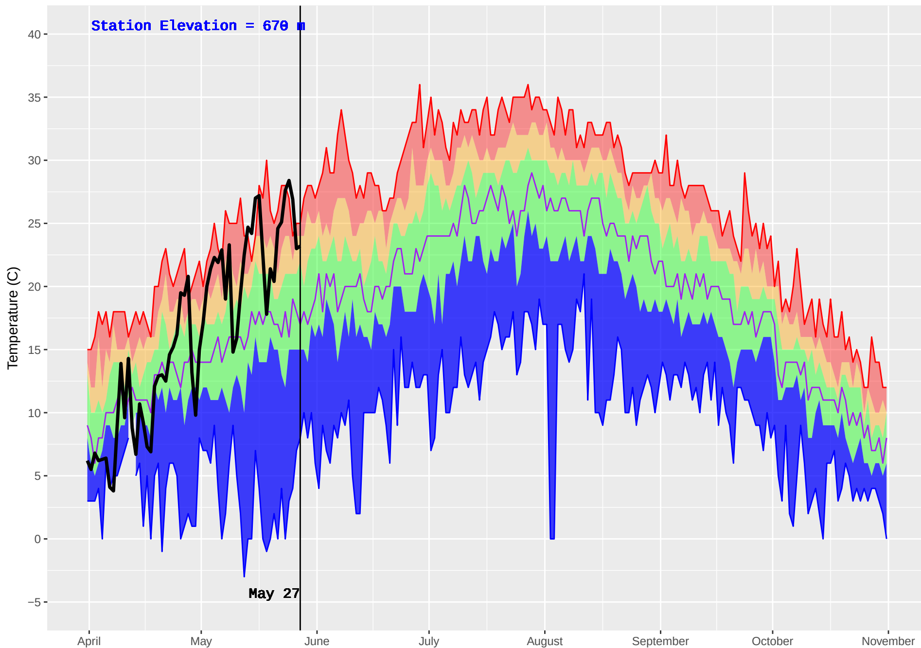
FINTRY (298) : Historical (1989–2016) and Current (2018) Noon Temperature
