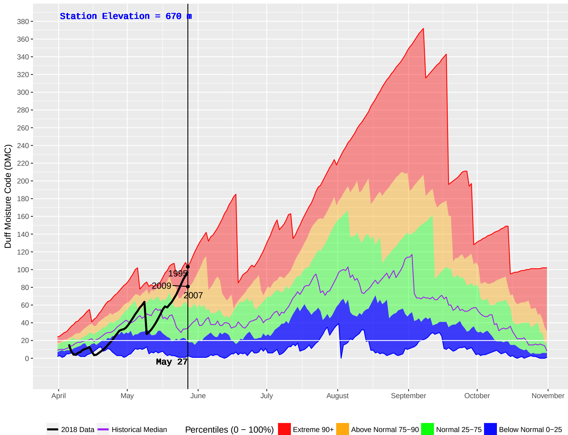
FINTRY (298) : Historical (1989–2016) and Current (2018) Noon Duff Moisture Code (DMC)
